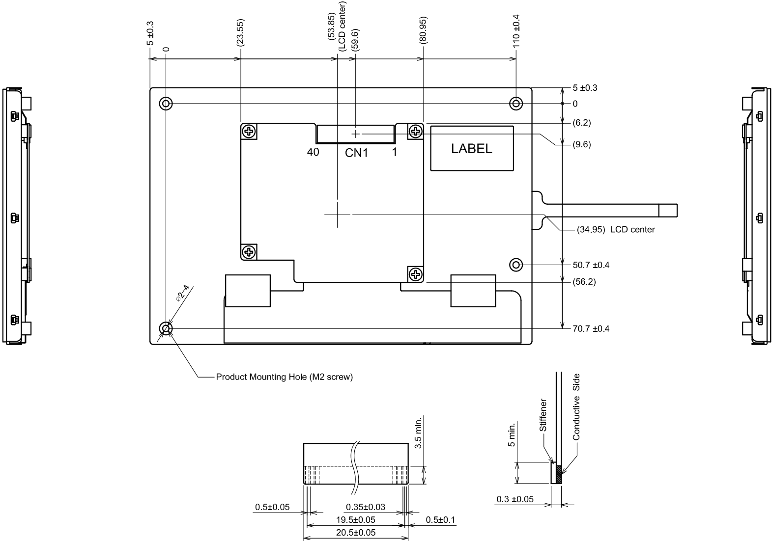
Recommended design rule for CN1 FPC
