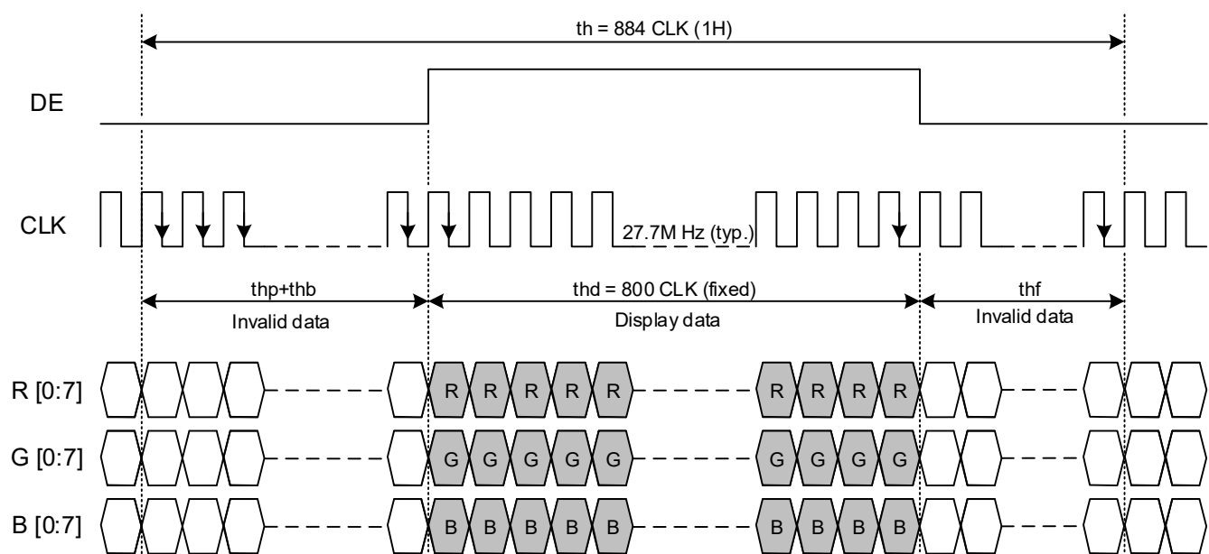
Fig. 8.1 Horizontal Timing
