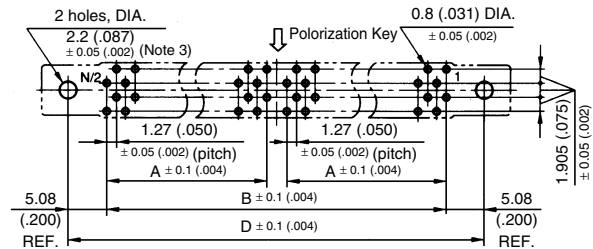
160, 200 Contacts
