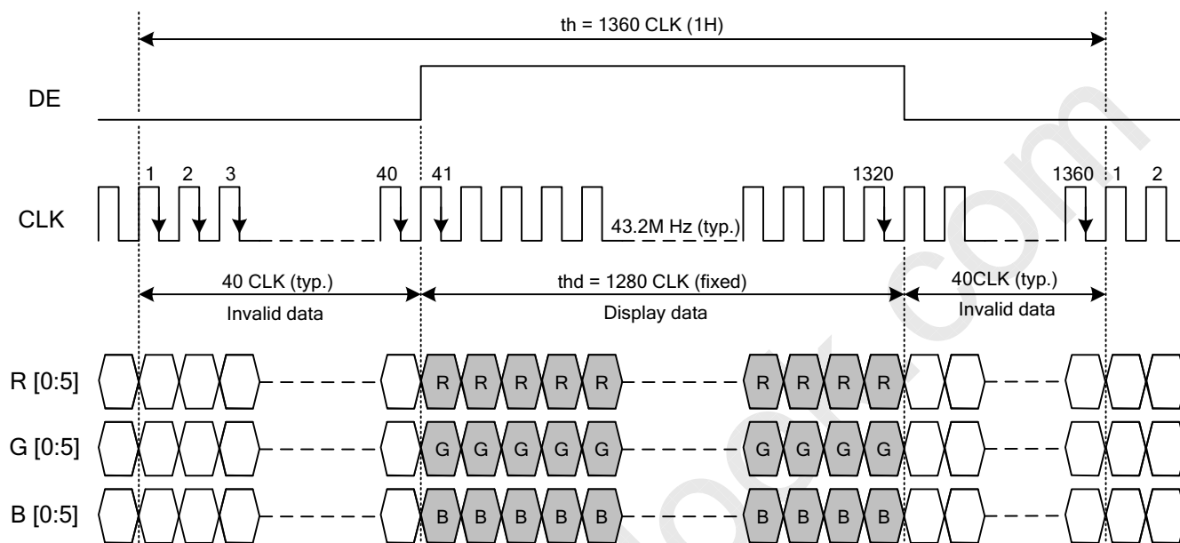
Fig. 8.3 Horizontal Timing
