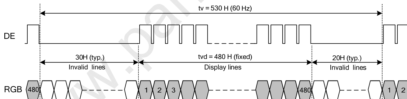
Fig. 8.4 Vertical Timing
