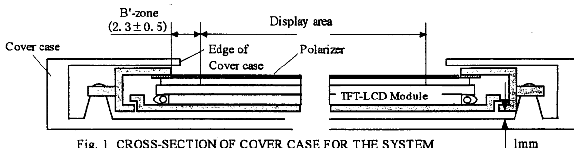
Fig. 1 CROSS-SECTION OF COVER CASE FOR THE SYSTEM
