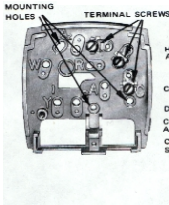
FIGURE 2 SUBBASE
