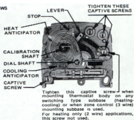
FIGURE 3 THERMOSTAT BODY
