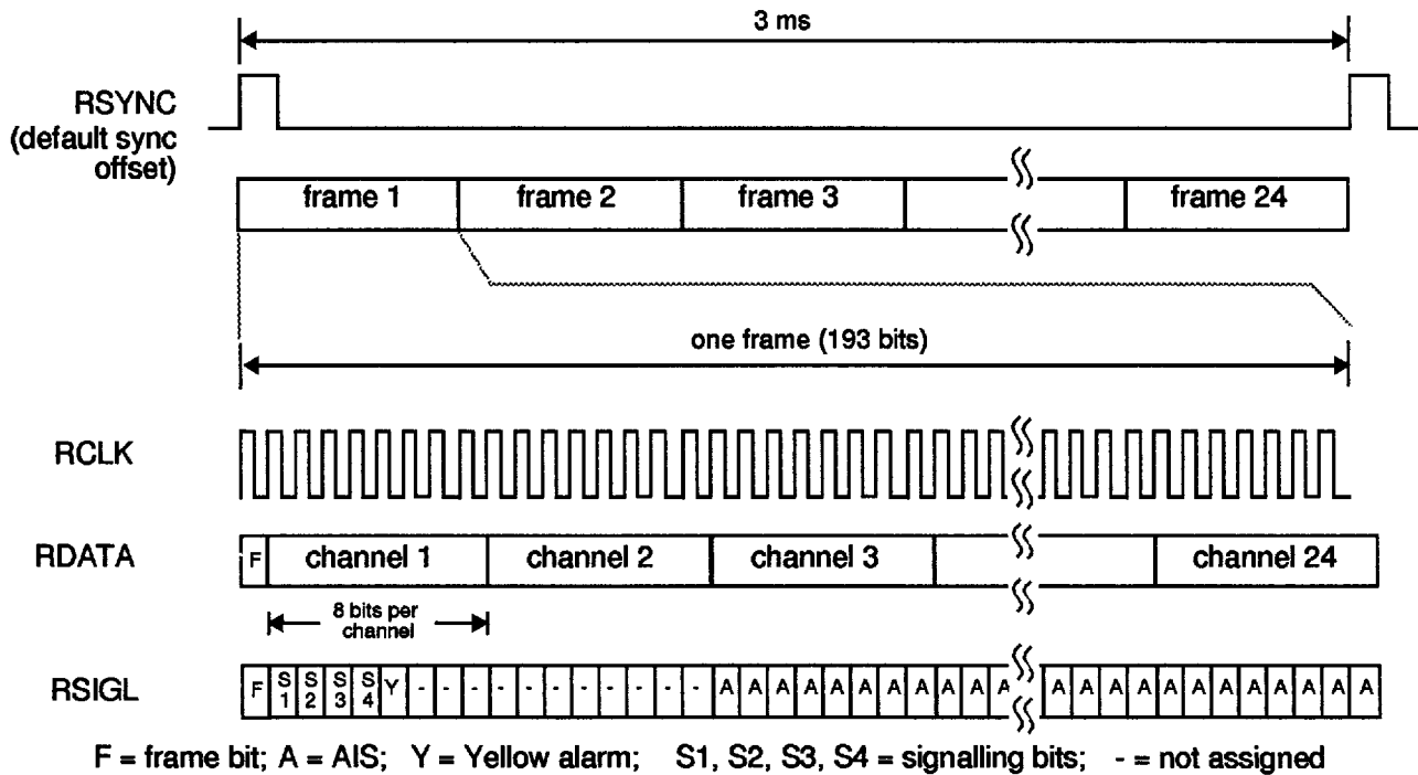
Figure 5. System Interface Receive Framing Format for Transmission Mode
