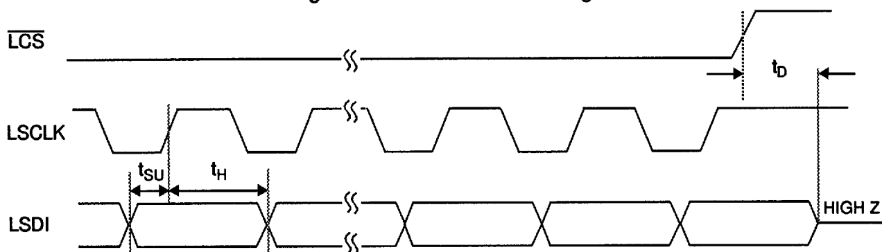
Figure 17. Serial Port Read Timing
