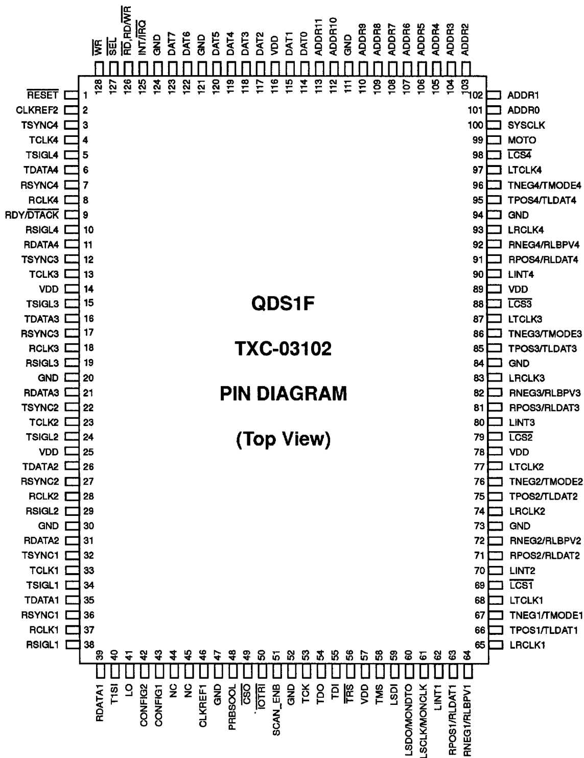
Figure 13. QDS1F TXC-03102 Pin Diagram
