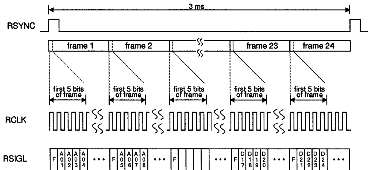
Figure 6. System Interface Receive Signaling Format for Transmission Mode
