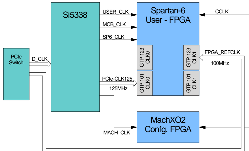
Figure 7-5 : FPGA Clock Sources
