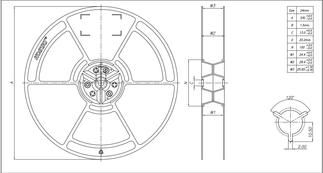
Figure 8. Plastic reel
