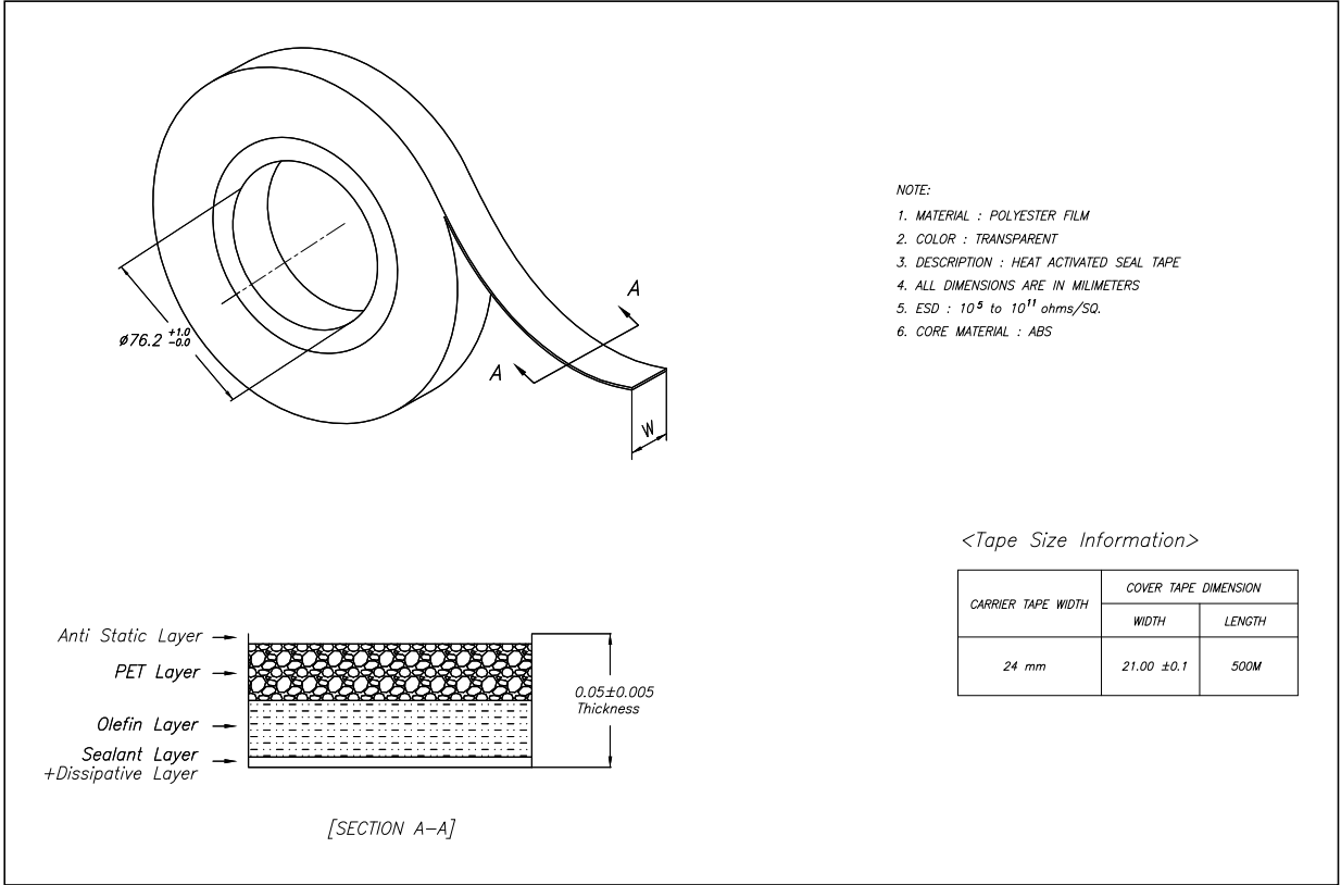
Figure 7. Cover tape
