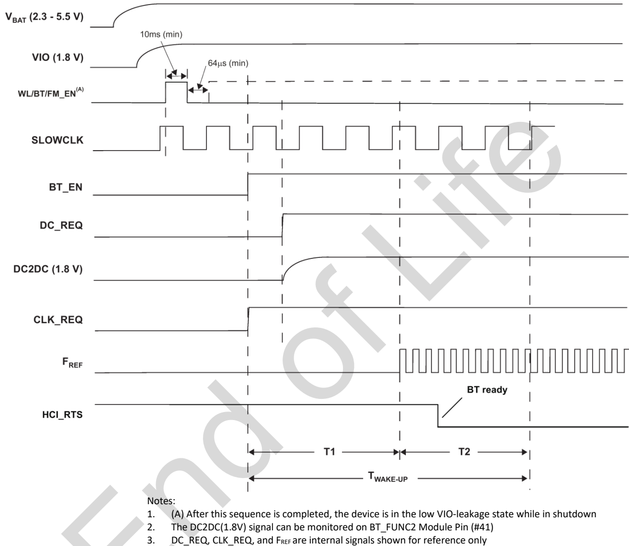
Figure 5 Bluetooth Power-up Sequence
