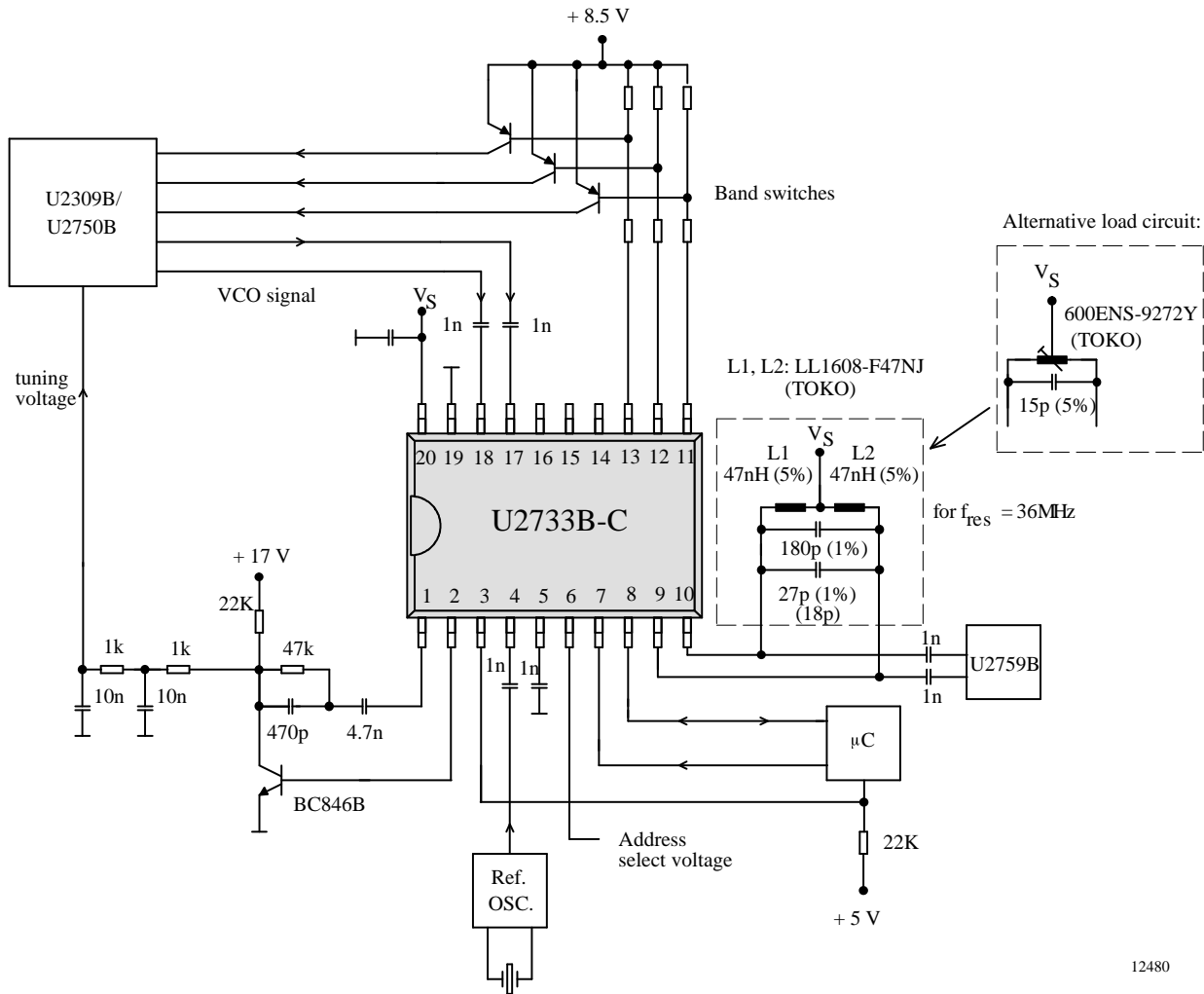
Figure 6. Application circuit
