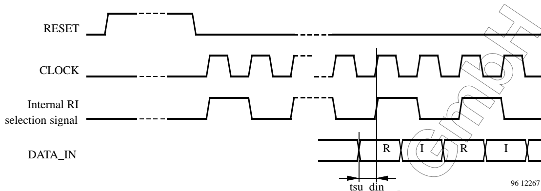
Figure 3. Input interface signals ( tsu\_din \geq 10\text{ ns} )
