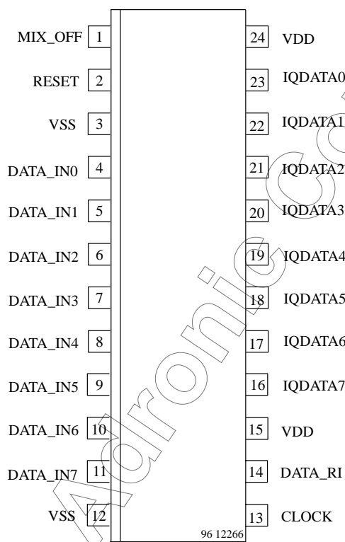
Figure 2. Pinning
