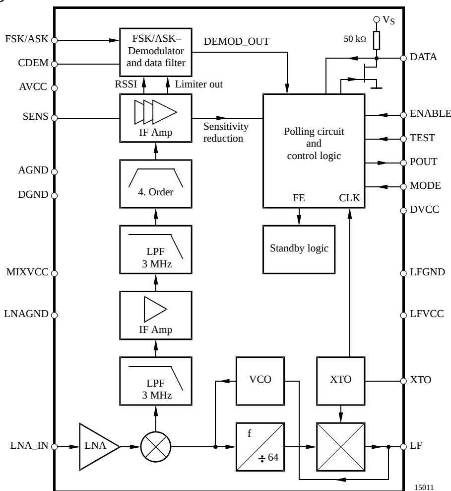
Figure 3. Block diagram
