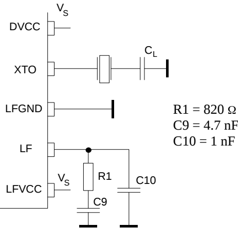
Figure 4. PLL peripherals
