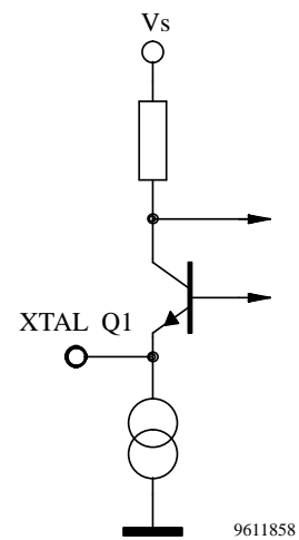
Figure 11. Reference oscillator
