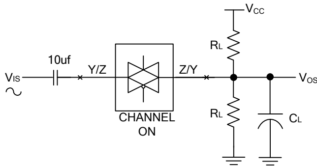
Fig. 6 Sine-Wave Distortion
