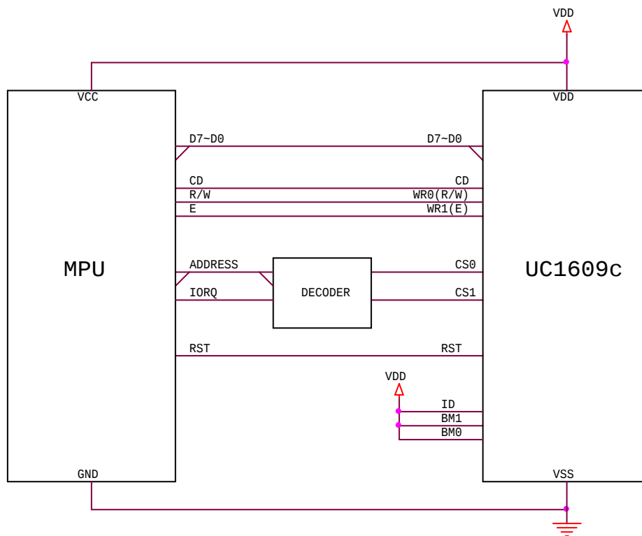
FIGURE 7: 6800/8bit parallel mode reference circuit
