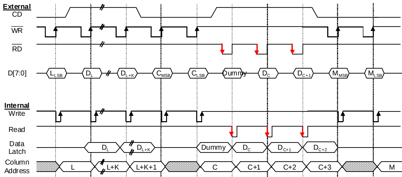
Figure 3: Parallel Interface & Related Internal Signals
