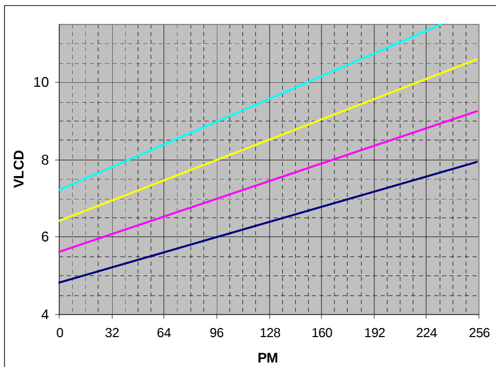
V LCD Programming Curve.
