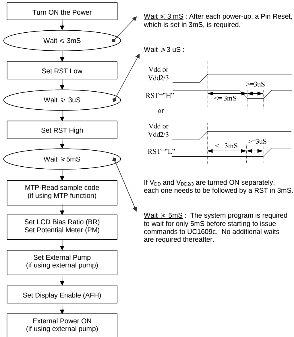
FIGURE 11: Reference Power-Up Sequence
