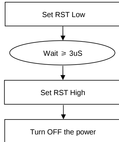
FIGURE 14: Reference Power-Down Sequence
