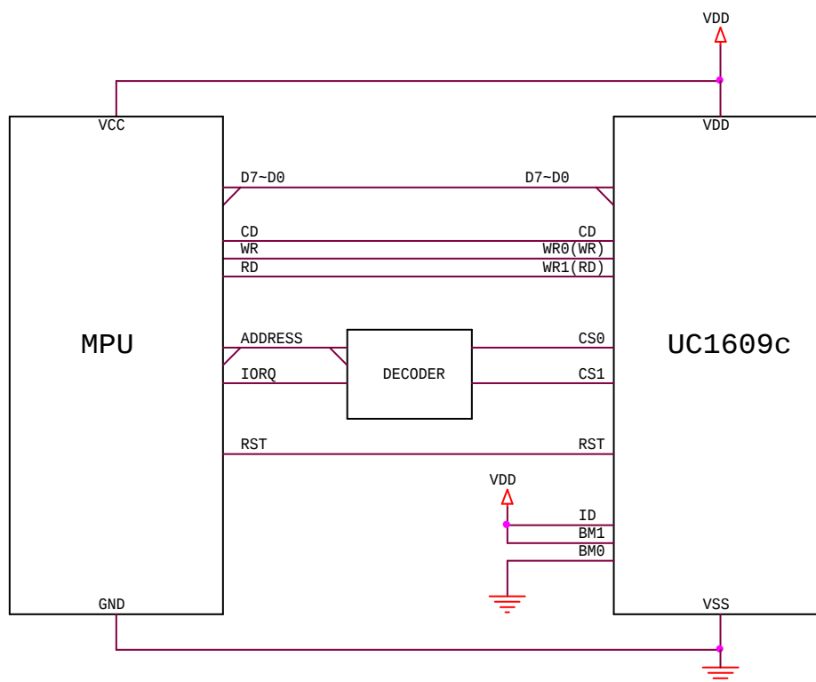
FIGURE 6: 8080/8bit parallel mode reference circuit
