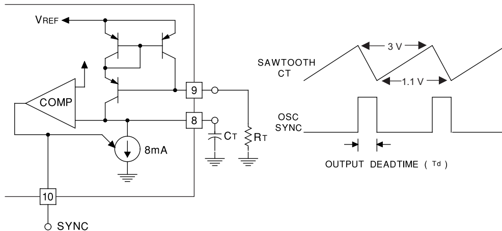
Figure 7. Oscillator Circuit
