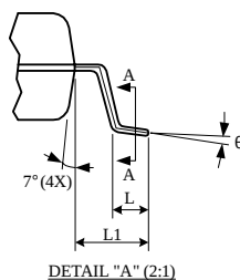
DETAIL "A" (2:1)
