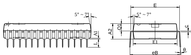
PDIP - 28
