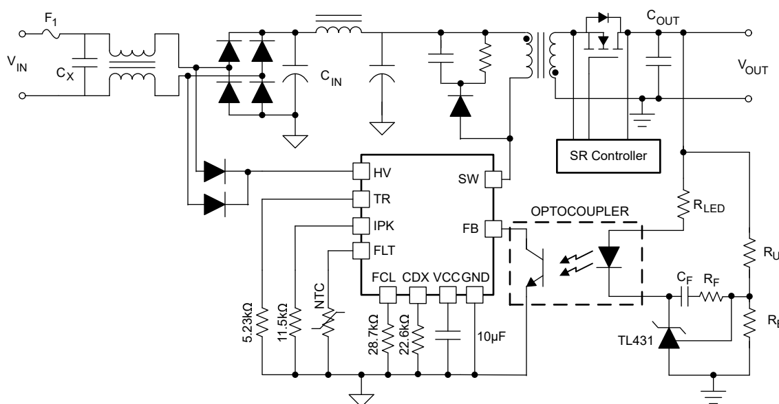
Figure 8-1. Typical Application Schematic
