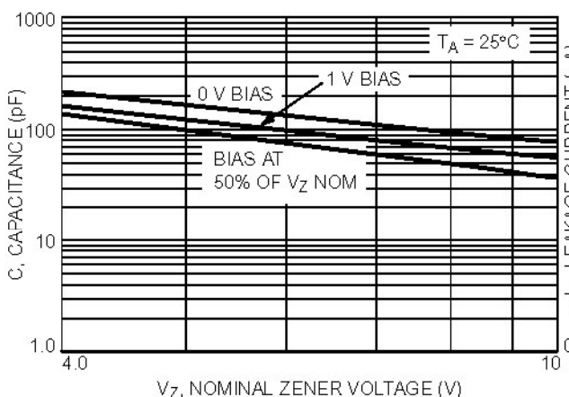
Figure 3. Typical Capacitance
