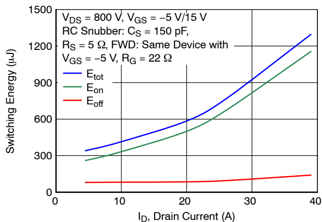
Figure 19. Clamped Inductive Switching Energy vs. Drain Current at T_J = 25^\circ\text{C} , Turn-on R_{G\_EXT} = 1 \Omega , and Turn-off R_{G\_EXT} = 22 \Omega
