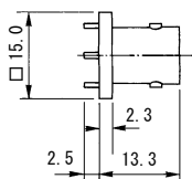
PCB Mounting Dimensions
