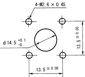
Mounting Hole
