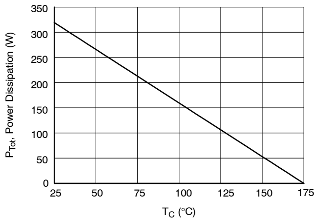
Figure 4. Power Dissipation
