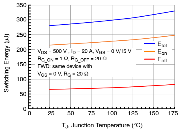
Figure 24. Clamped Inductive Switching Energy vs. Junction Temperature at V_{DS} = 500 V, and I_D = 20 A
