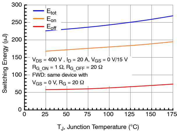
Figure 23. Clamped Inductive Switching Energy vs. Junction Temperature at V_{DS} = 400 V, and I_D = 20 A
