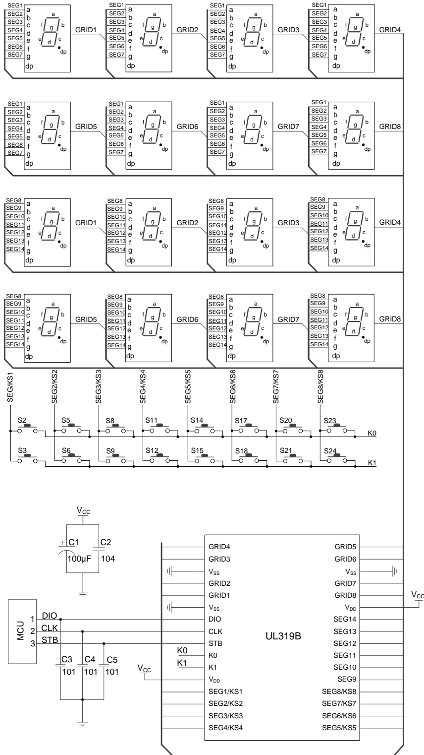
UL319B driver Common cathode digital screen hardware circuit
