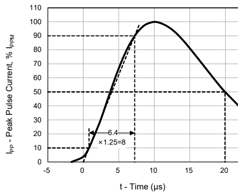
Fig.3 - 8/20 \mu\text{s} Pulse Waveform
