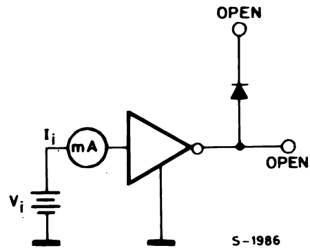
Figure 6. Input current (ON)
