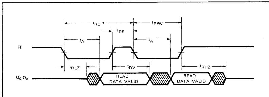
Figure 3. Asynchronous Read Operation
