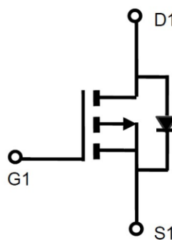
P-Channel
