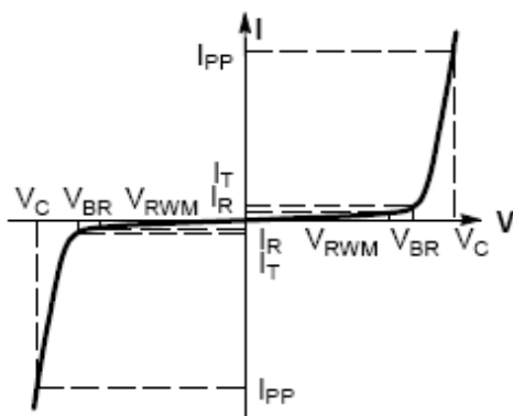
Bi-Directional TVS
