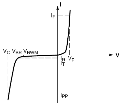
Uni-Directional TVS
