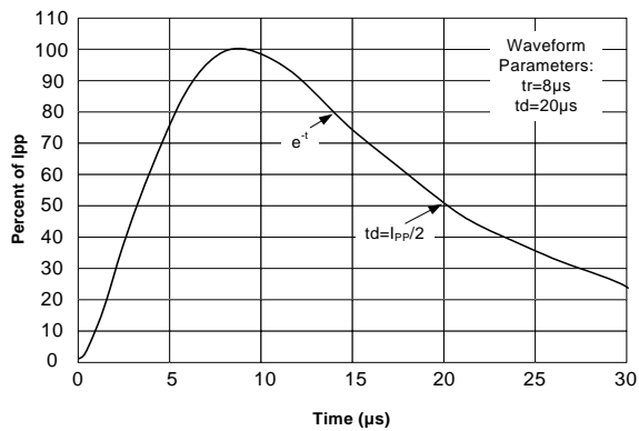
Pulse Waveform
