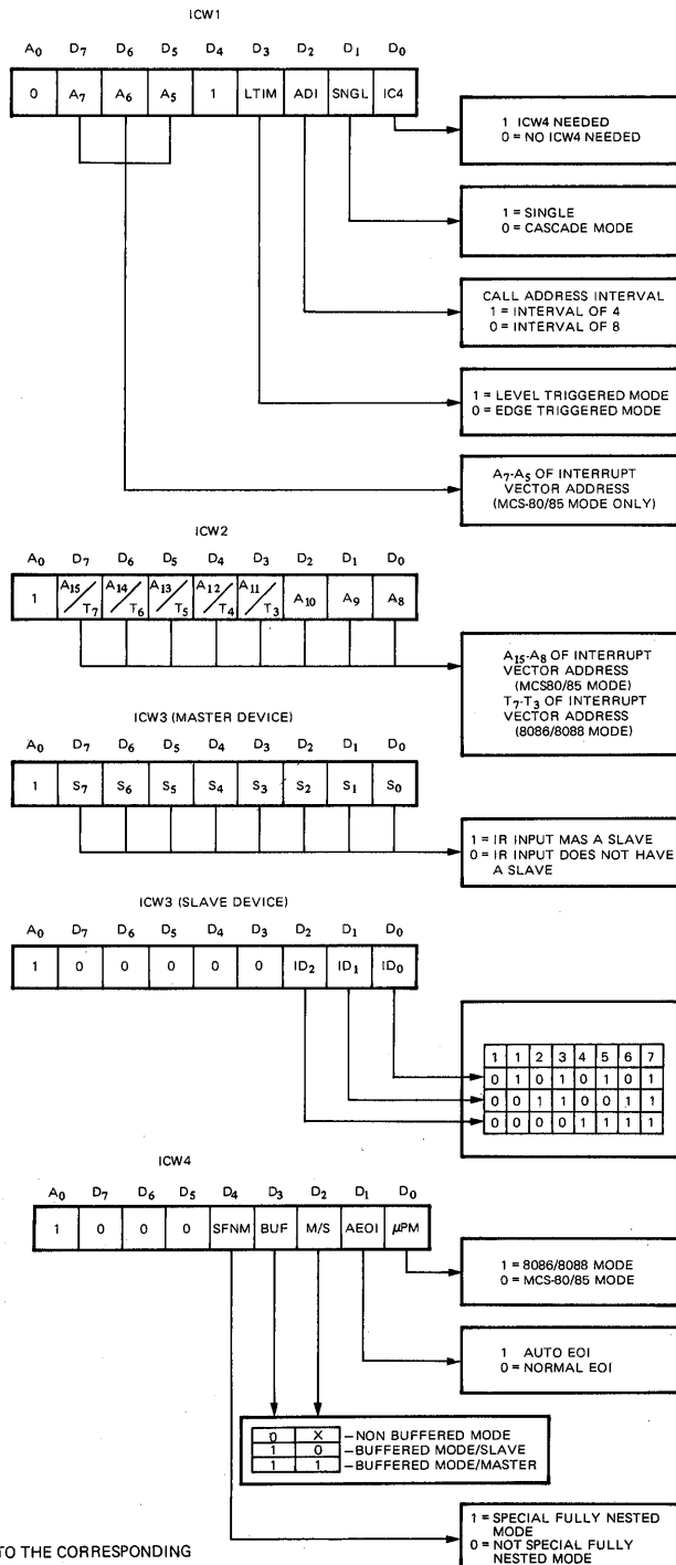
Figure 5. Initialization Command Word Format
