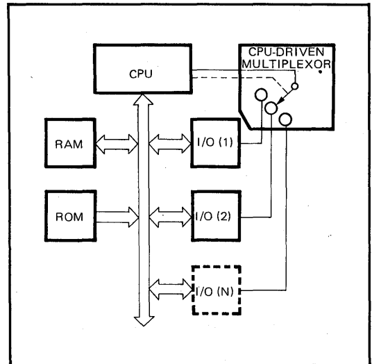
Figure 1a. Polled Method
