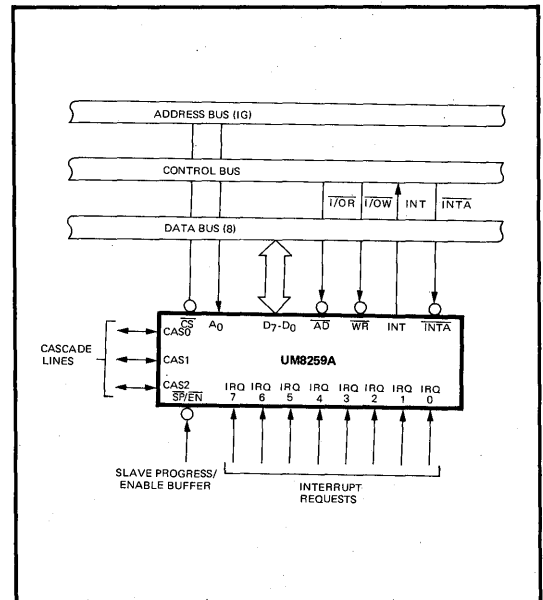
Figure 3. UM8259A Interface to Standard System Bus
