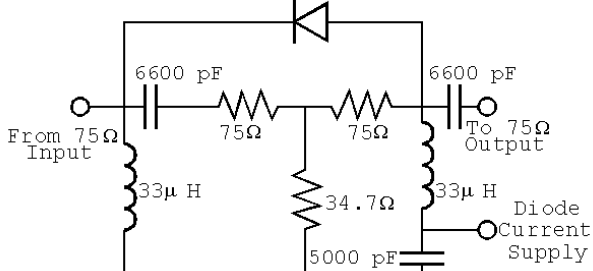
TEST CIRCUIT FOR DISTORTION MEASUREMENTS D.U.T.
