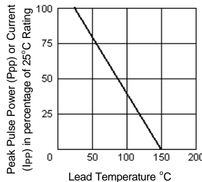
FIGURE 3 Derating Curve
