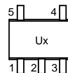
SC-88A/SOT-323 CASE 419A STYLE 6
