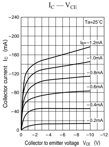
Characteristics charts of UN612Y
