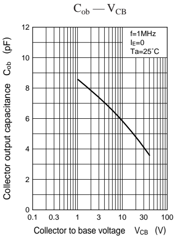
Characteristics charts of UN6224
