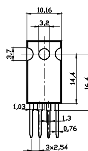
USR 4-T221 / UNR 4-T221
