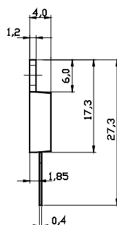
USR 4-T220B / UNR 4-T220B
