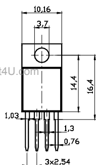
USR 4-T220B / UNR 4-T220B
