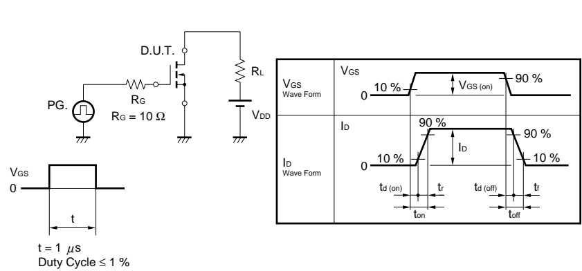
Test Circuit 2 Switching Time
