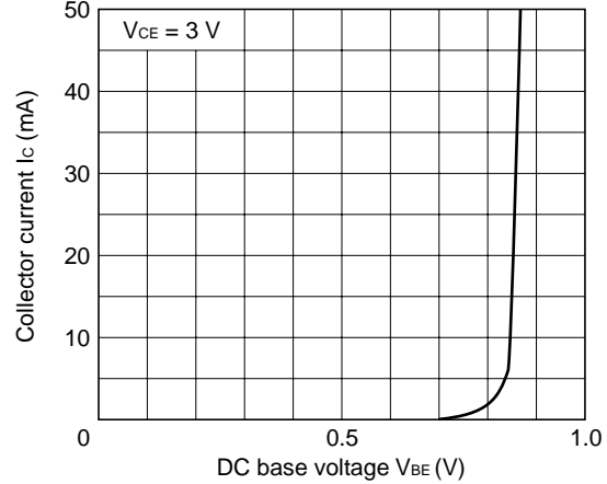
Collector Current vs. DC Base Voltage
