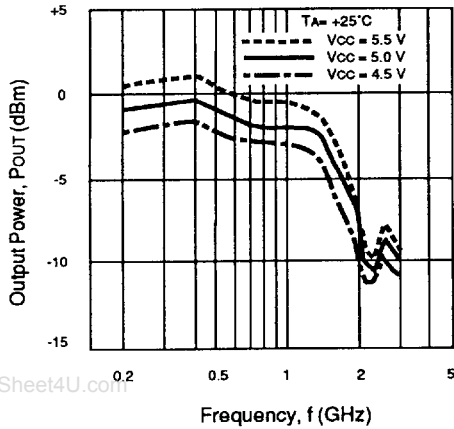
OUTPUT POWER vs. FREQUENCY AND VOLTAGE
