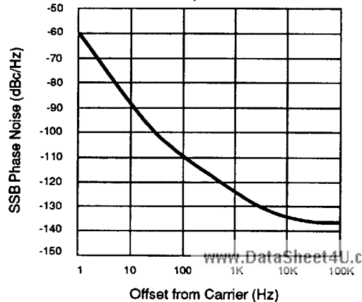
UPB584G SSB PHASE NOISE vs. OFFSET FROM CARRIER fIN = 1 GHz, TA = 25°C
