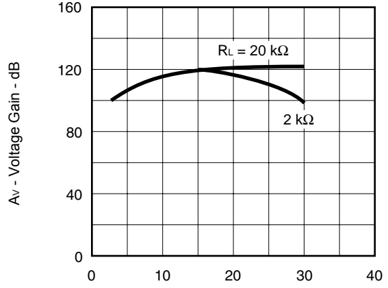
V^+ - Power Supply Voltage - V ( V^- = GND)
