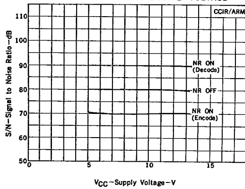
SIGNAL TO NOISE RATIO vs. SUPPLY VOLTAGE
