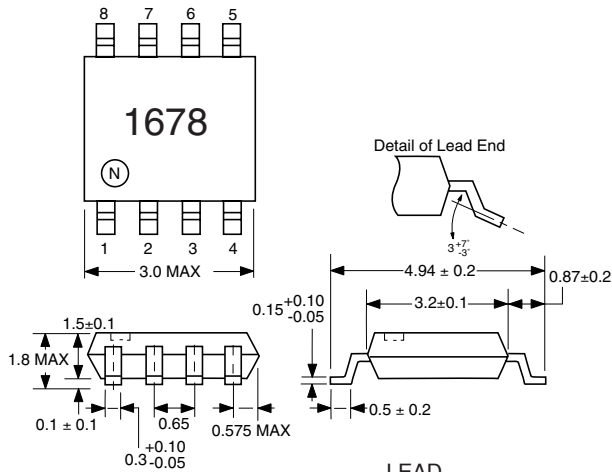
UPC1678GV PACKAGE OUTLINE S08
