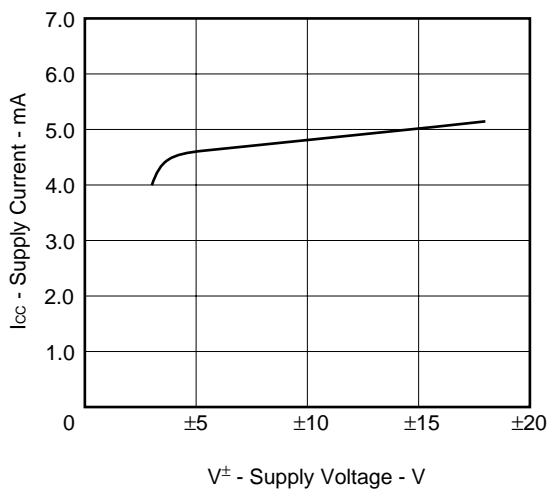
SUPPLY CURRENT
