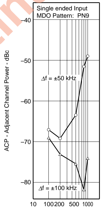
ACP vs V_{I/Qin} (at V_{CC} = 3.0 V)
