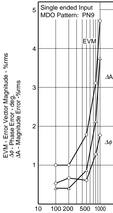
EVM, \Delta\phi , \Delta A vs V_{I/Qin} (at V_{CC} = 2.7 V)
