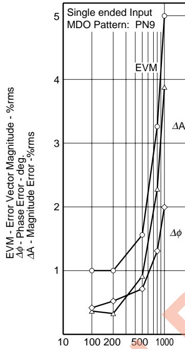
EVM, \Delta\phi , \Delta A vs V_{I/Qin} (at V_{CC} = 3.0 V)
