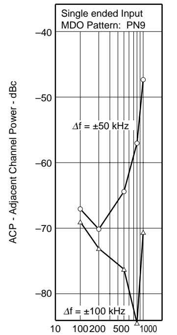
ACP vs V_{I/Qin} (at V_{CC} = 3.6 V)
