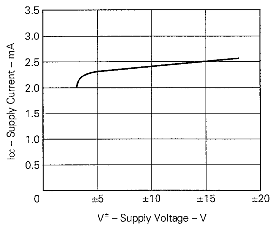
SUPPLY CURRENT
