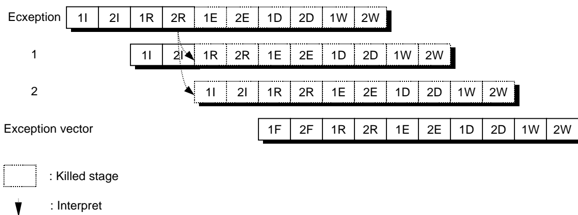
Figure 4-12. Exception Detection
