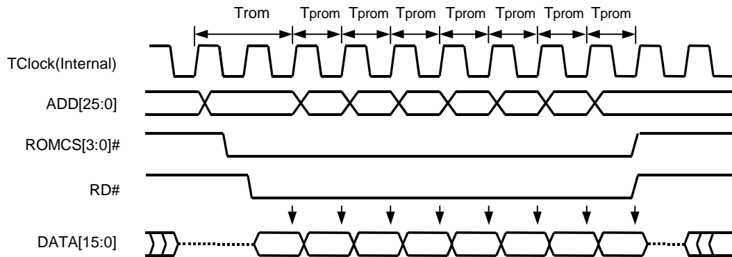
Figure 10-3. PageROM 4-word Read, 16-bit Mode (WROMA[2:0] = 111, WPROM[1:0] = 10)
