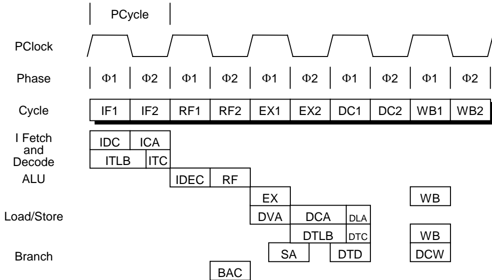
Figure 4-3. Pipeline Activities
