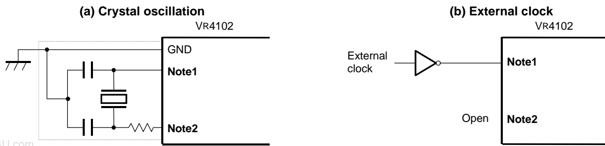
Figure 1-9. External Circuit of Clock Oscillator
