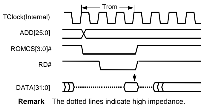
Figure 10-2. ROM 4-byte Read, 32-bit Mode (WROMA[2:0] = 110)
