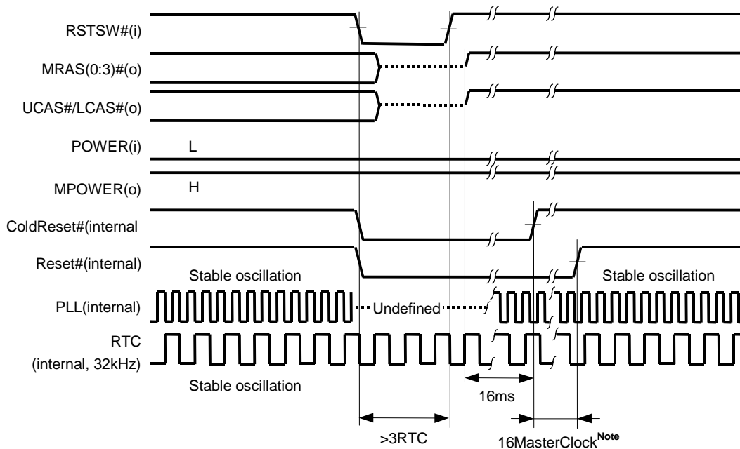
Figure 7-2. RSTSW
