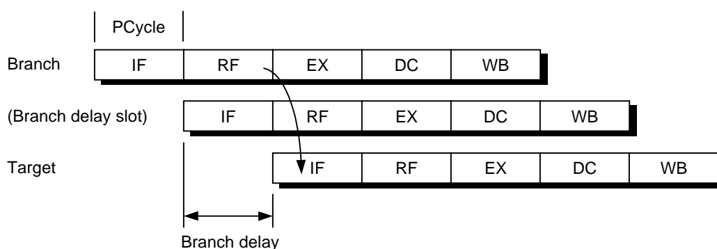
Figure 4-4. Branch Delay
