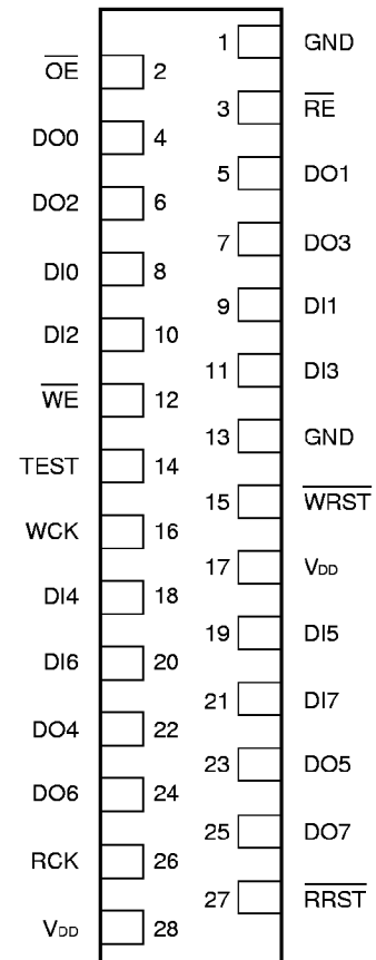
28-pin plastic ZIP (400 mil) (Bottom View) \mu PD42280V-xx
