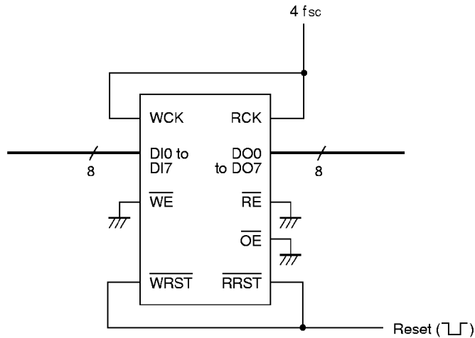
Figure 5-1 Circuit of 1 field delay line
