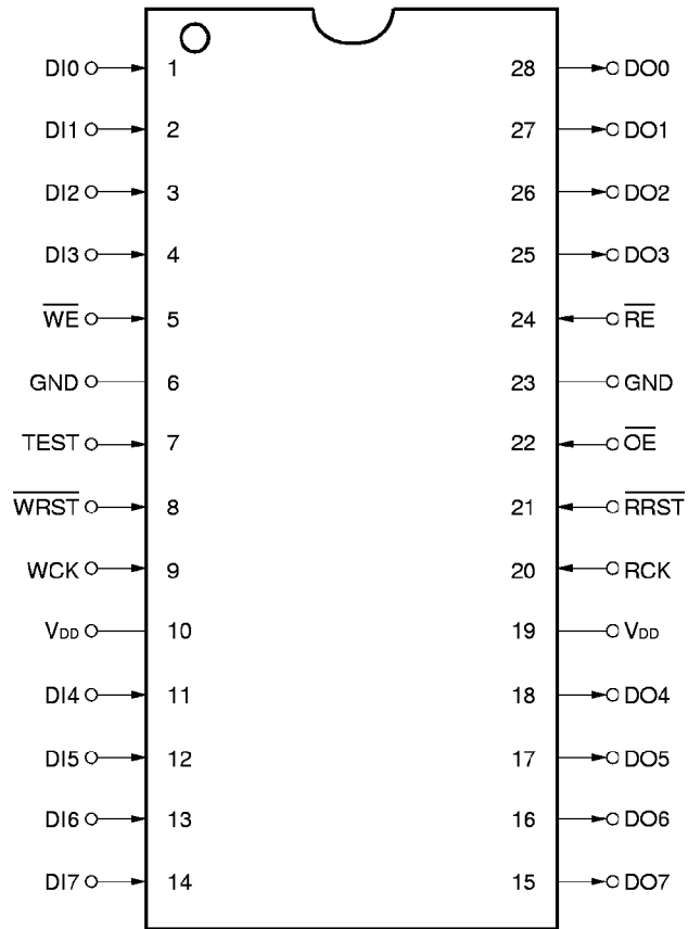
28-pin plastic SOP (450 mil) (Top View) \mu PD42280GU-xx
